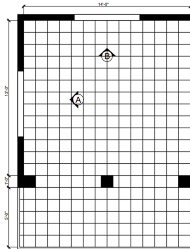
FLOOR PLAN SCALE: \frac{1}{4}" = 1'-0"
