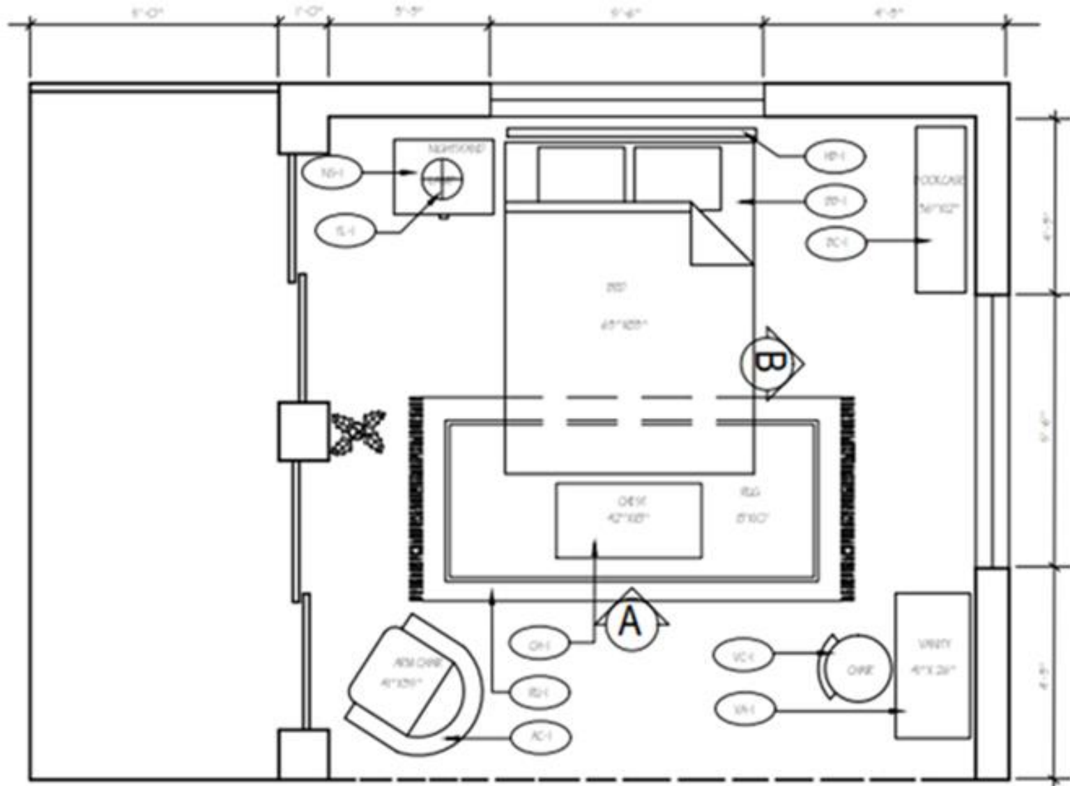
FLOOR PLAN/ BEDROOM SCALE 1/2" = 1'-0"
